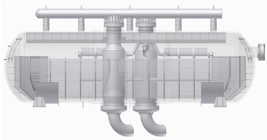
Figure 3. Loviisa powerplant horizontal steam generator
