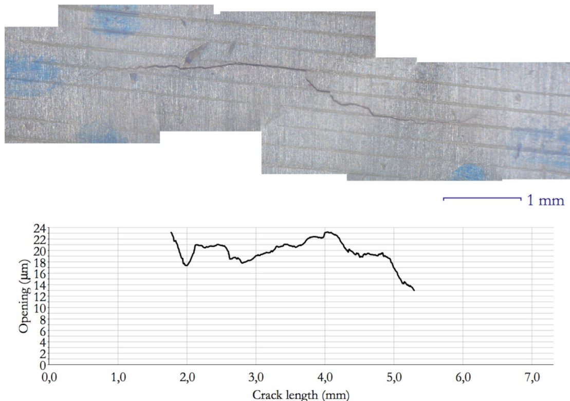
Figure 2. Example validation crack in E.On nozzle. Crack was imaged using a camera microscope and shown with respective crack opening measured from the image.
