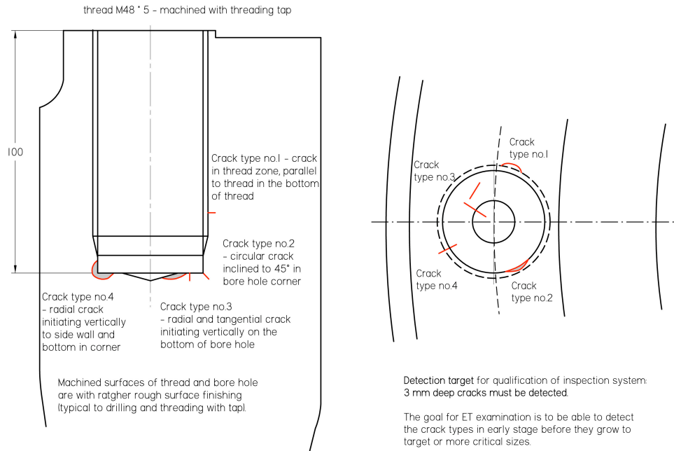
Figure 5. Flaw types to be detected in Loviisa primary collector qualification
