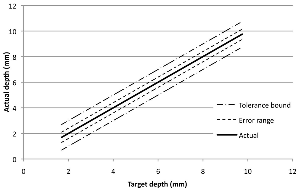
Figure 1. Example of validation data for austenitic stainless steel
